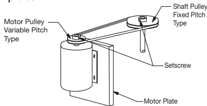
Figure 5 — Drive Package Diagram
