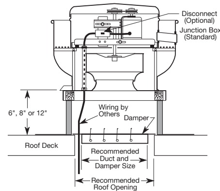
Figure 2 — Typical Roof-Mount
