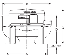
Figure 1 — Dimensions
