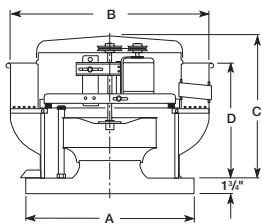
Figure 1 — Dimensions
